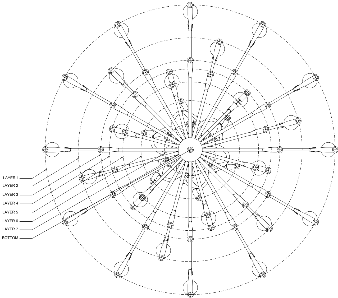
BOTTOM VIEW
